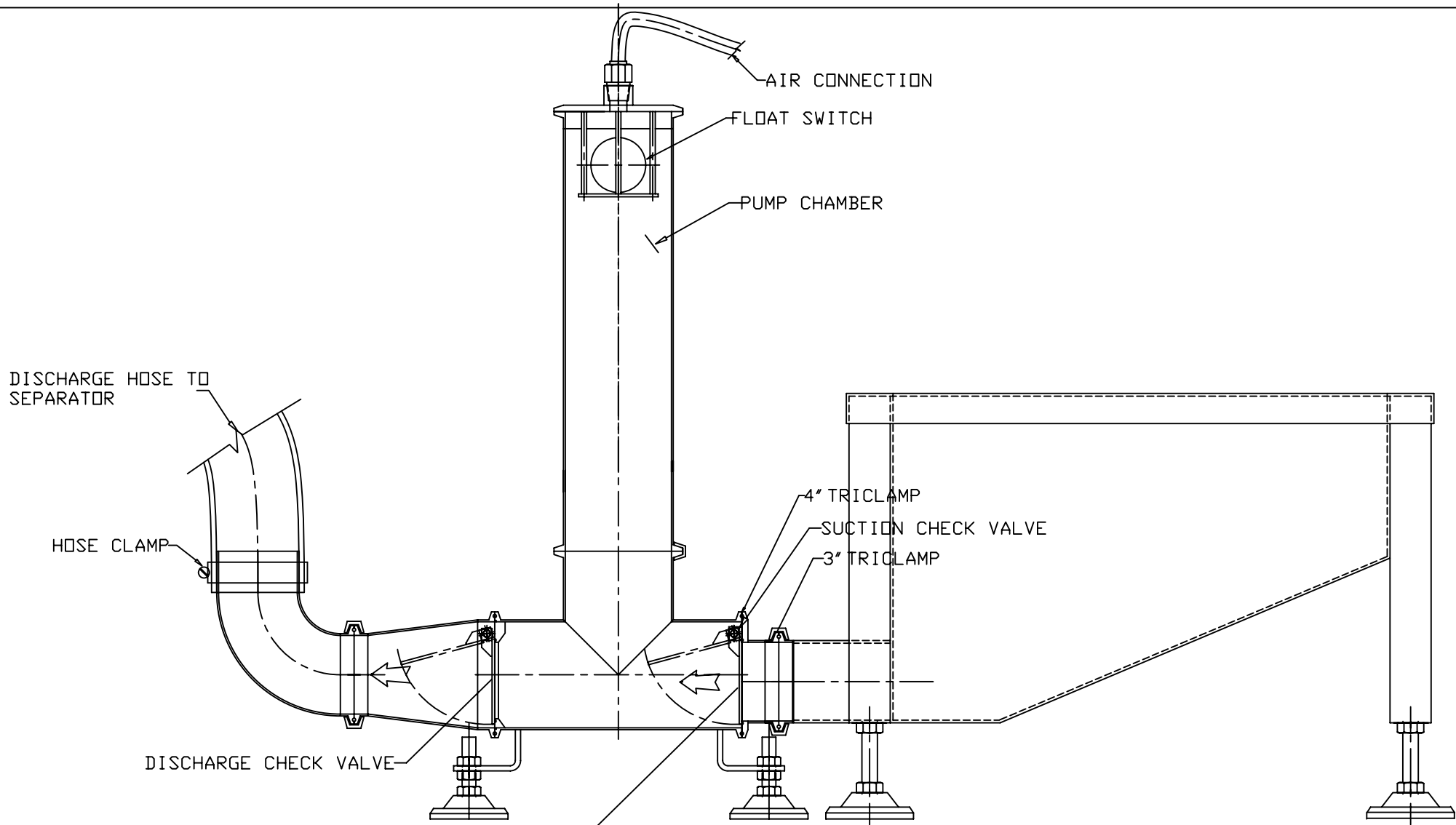
SIDE ELEVATION
