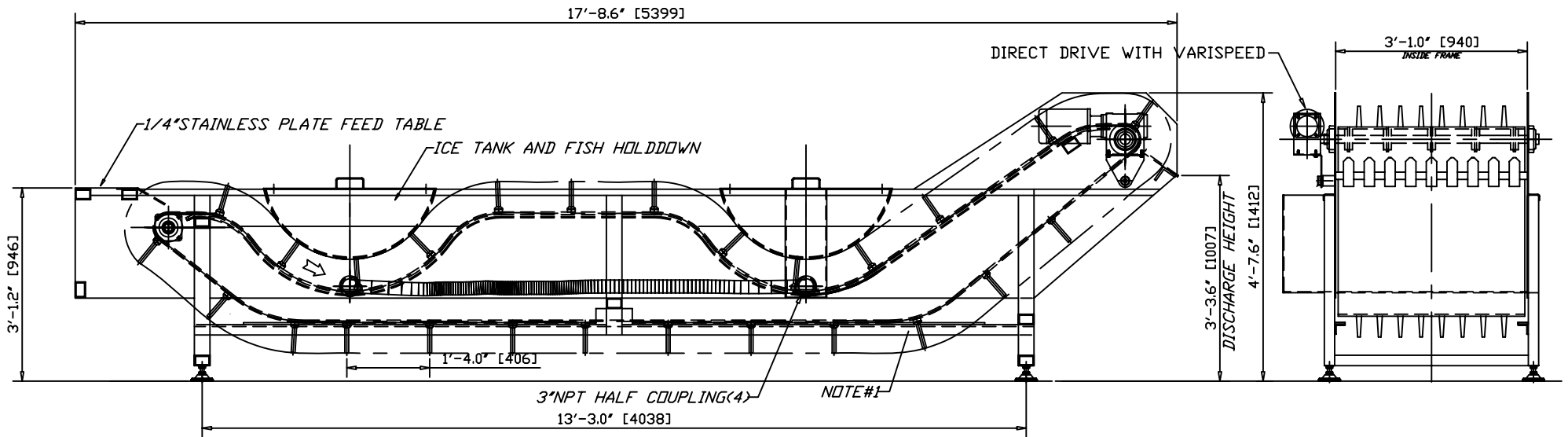
SIDE ELEVATION
